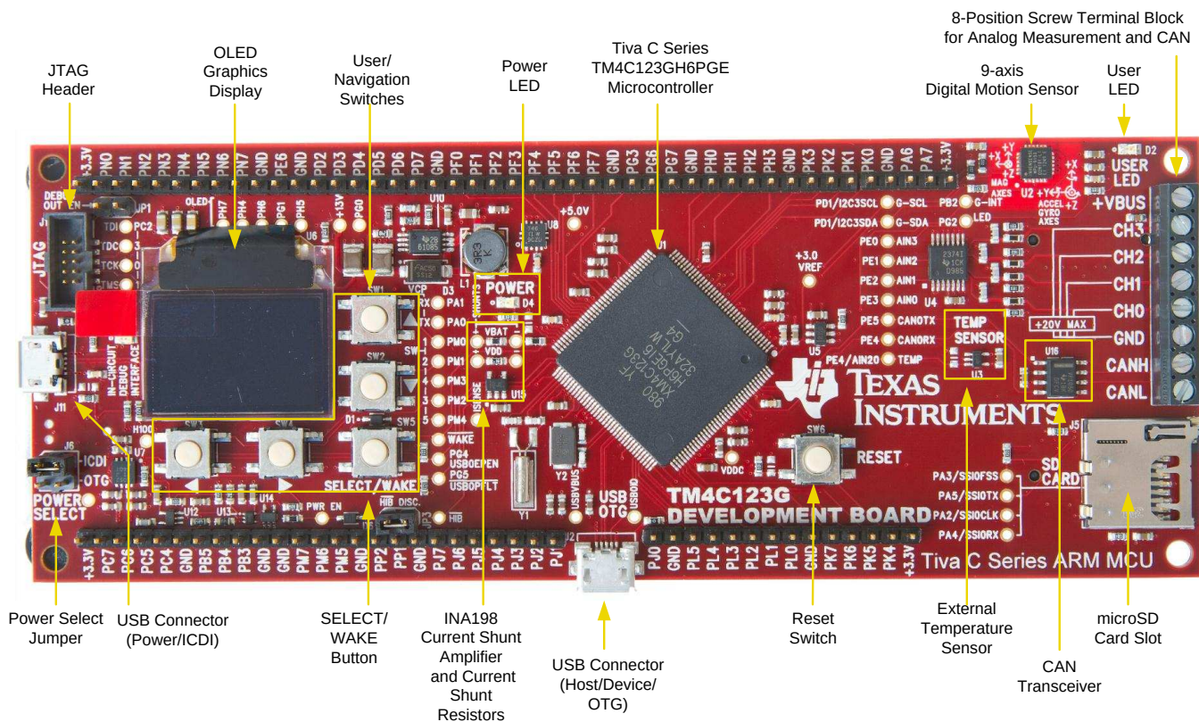
Figure 1-1. Board Picture
